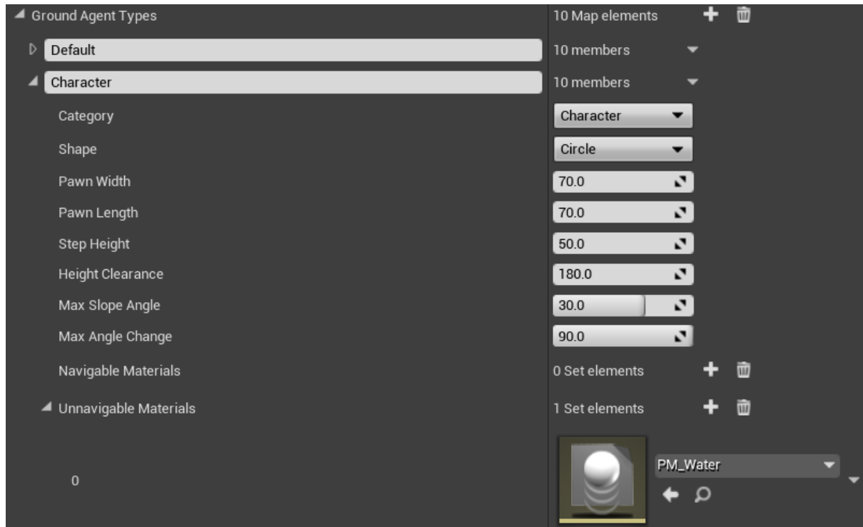
Configurable Agent Type properties
